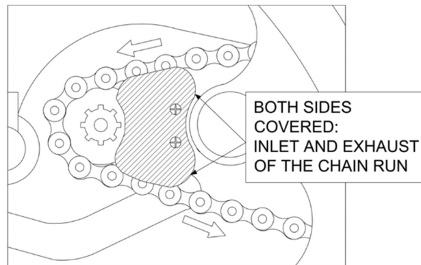
Figure 4 : Front sprocket protection
