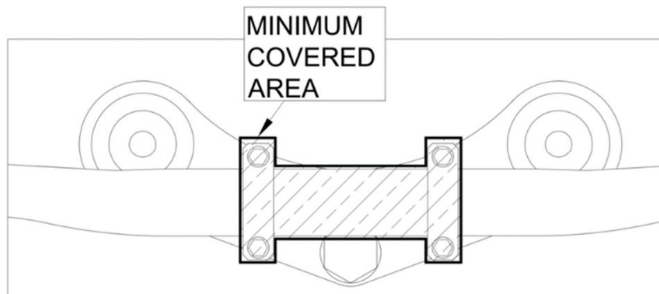
Figure 2 : Handlebar covering
