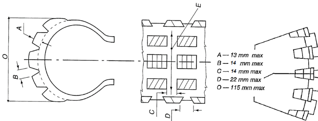
Figure 3 : Tyre dimensions
